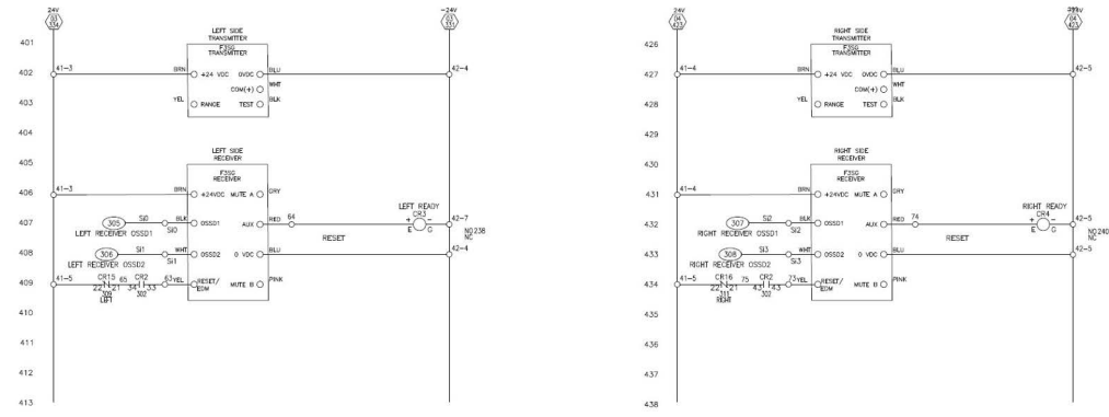
Figure 11: Updated Light Curtain Wiring
