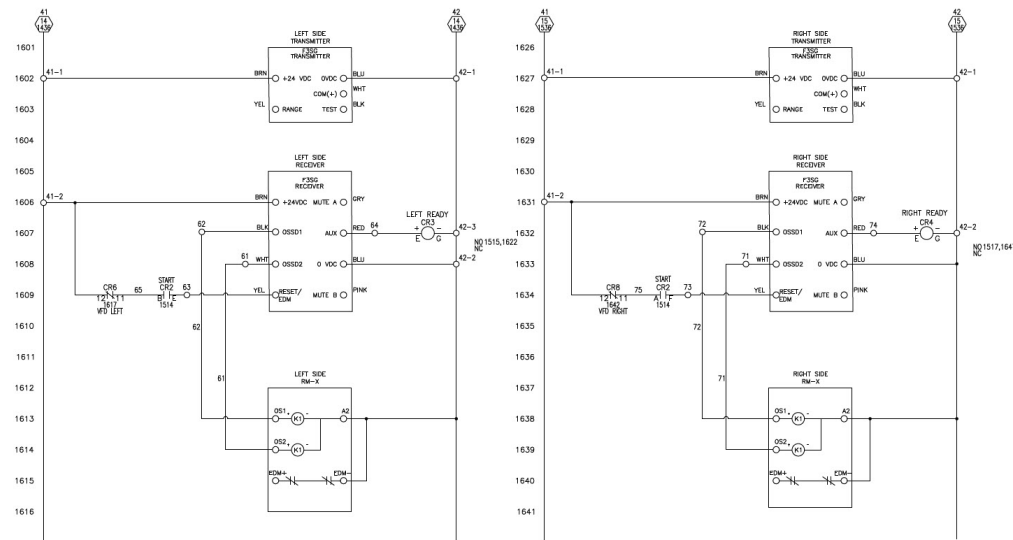
Figure 10: Updated Light Curtain Wiring
