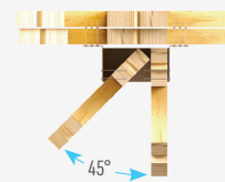
Typical HJC installation top view
