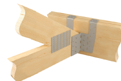
Typical MSHA29L top-max installation
