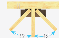
Typical HJHC installation top view
