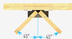
Typical HHC installation top view
