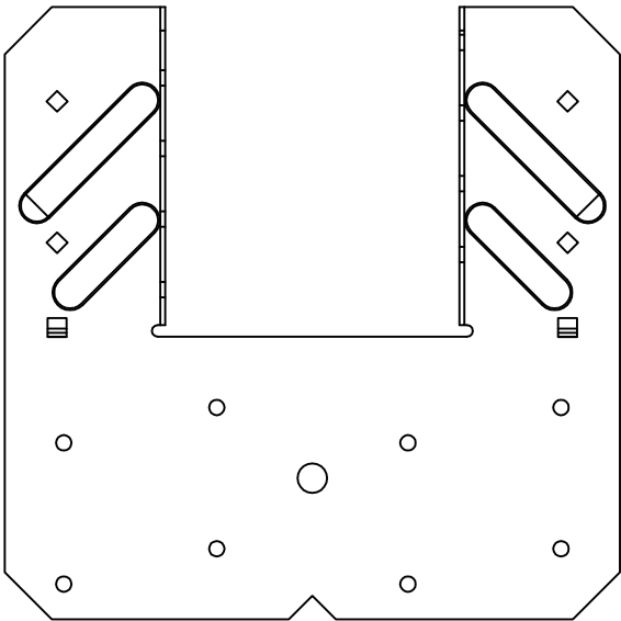
RT16-2 - FRONT VIEW
