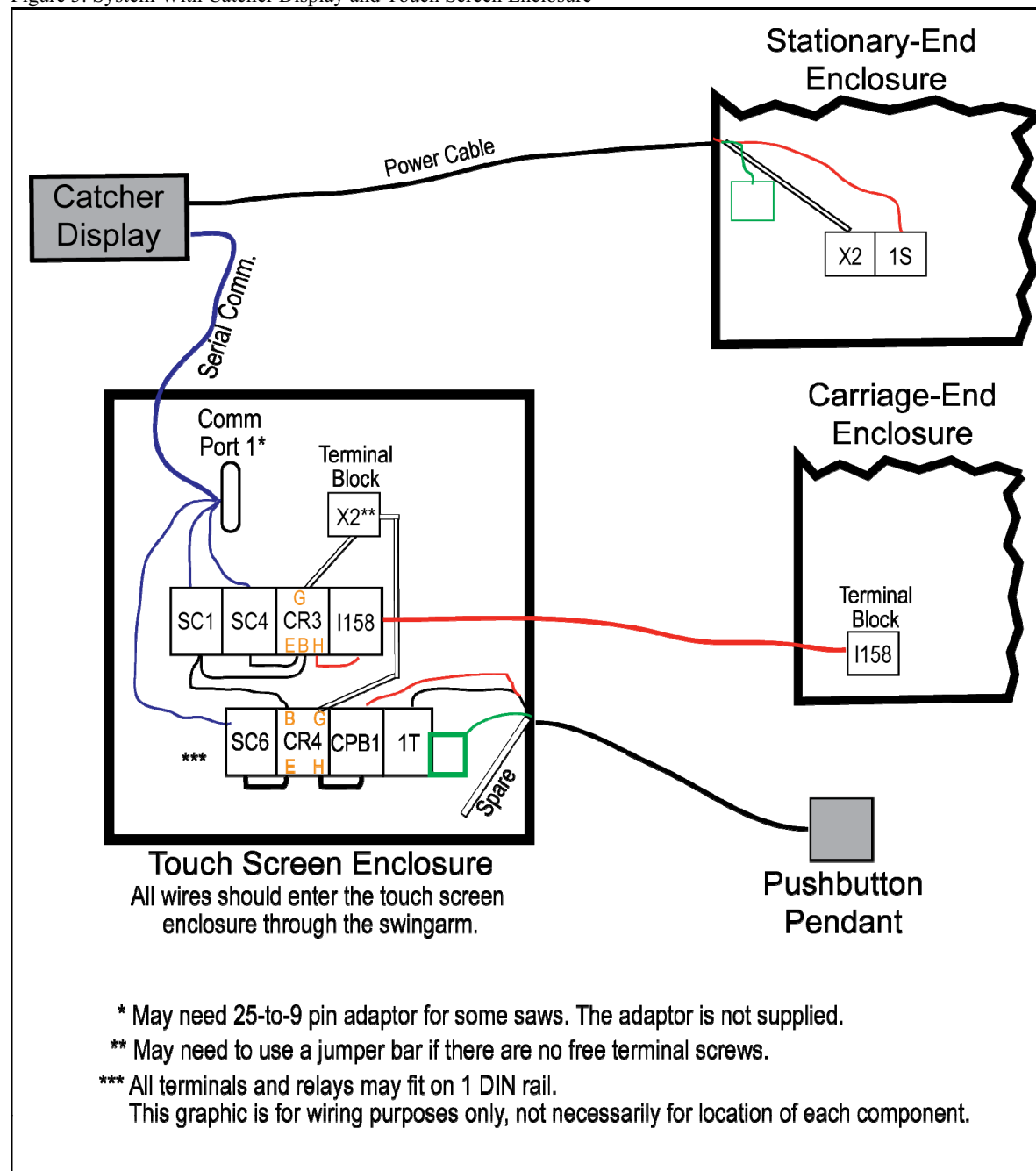
Figure 3: System With Catcher Display and Touch Screen Enclosure
