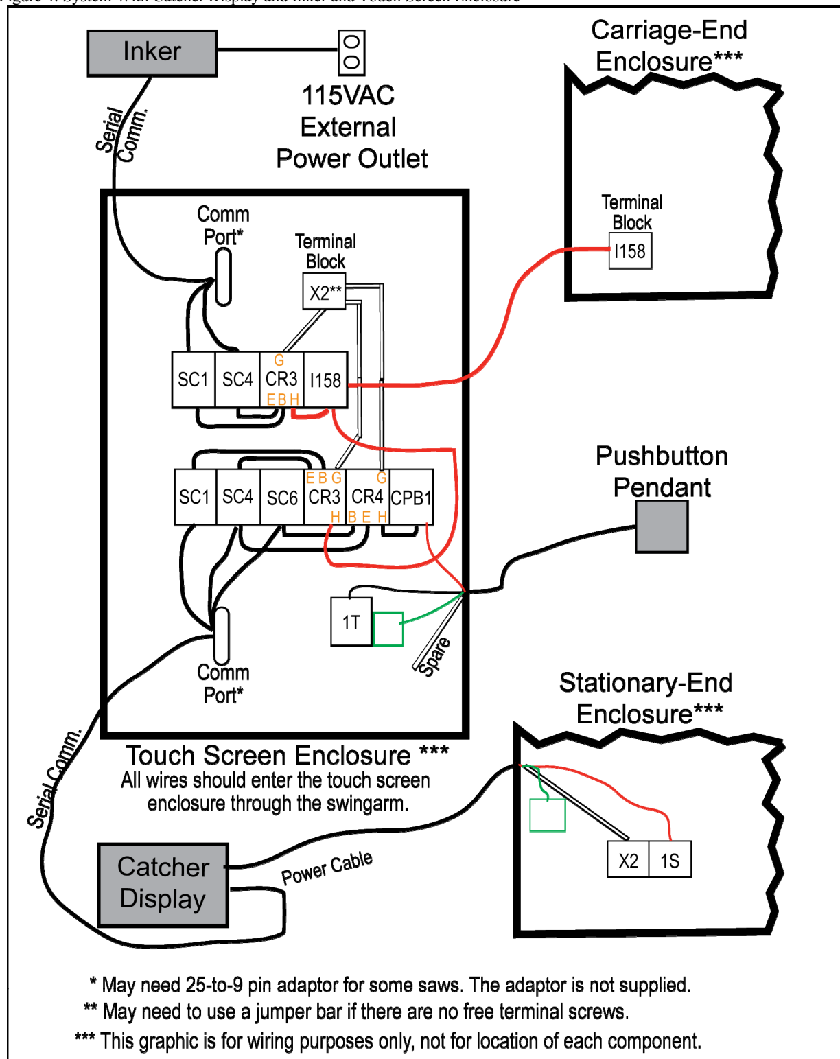
Figure 4: System With Catcher Display and Inker and Touch Screen Enclosure
