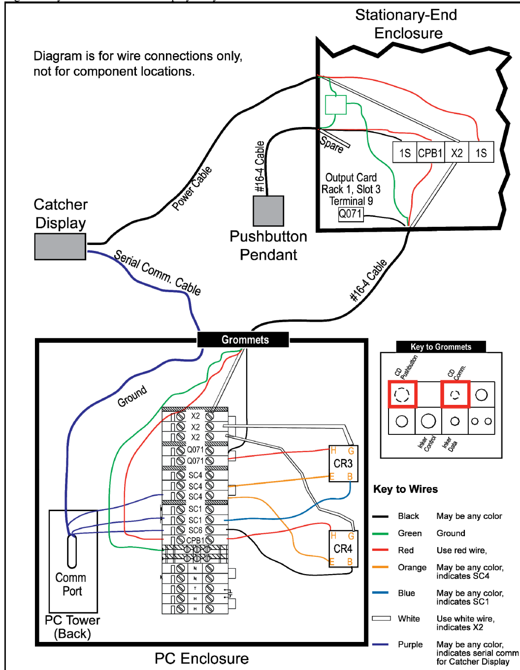
Figure 1: System With Catcher Display Only and PC Enclosure
