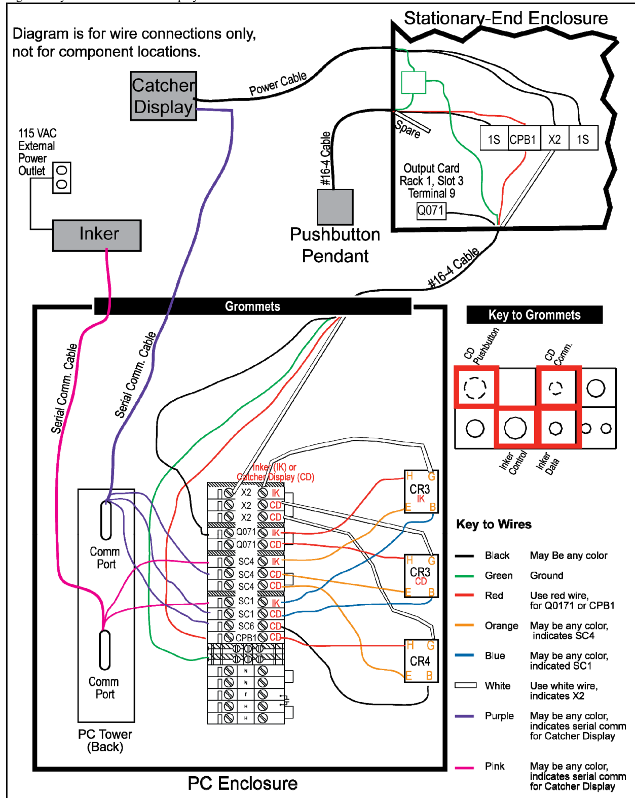
Figure 2: System With Catcher Display and Inker and a PC Enclosure
