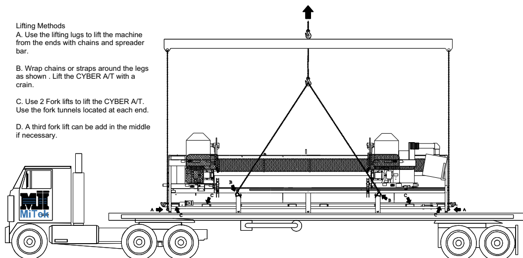
Figure 3-1: Lifting Methods
