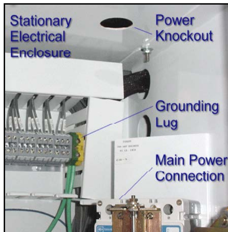
Figure 3-17: Disconnect Enclosure
