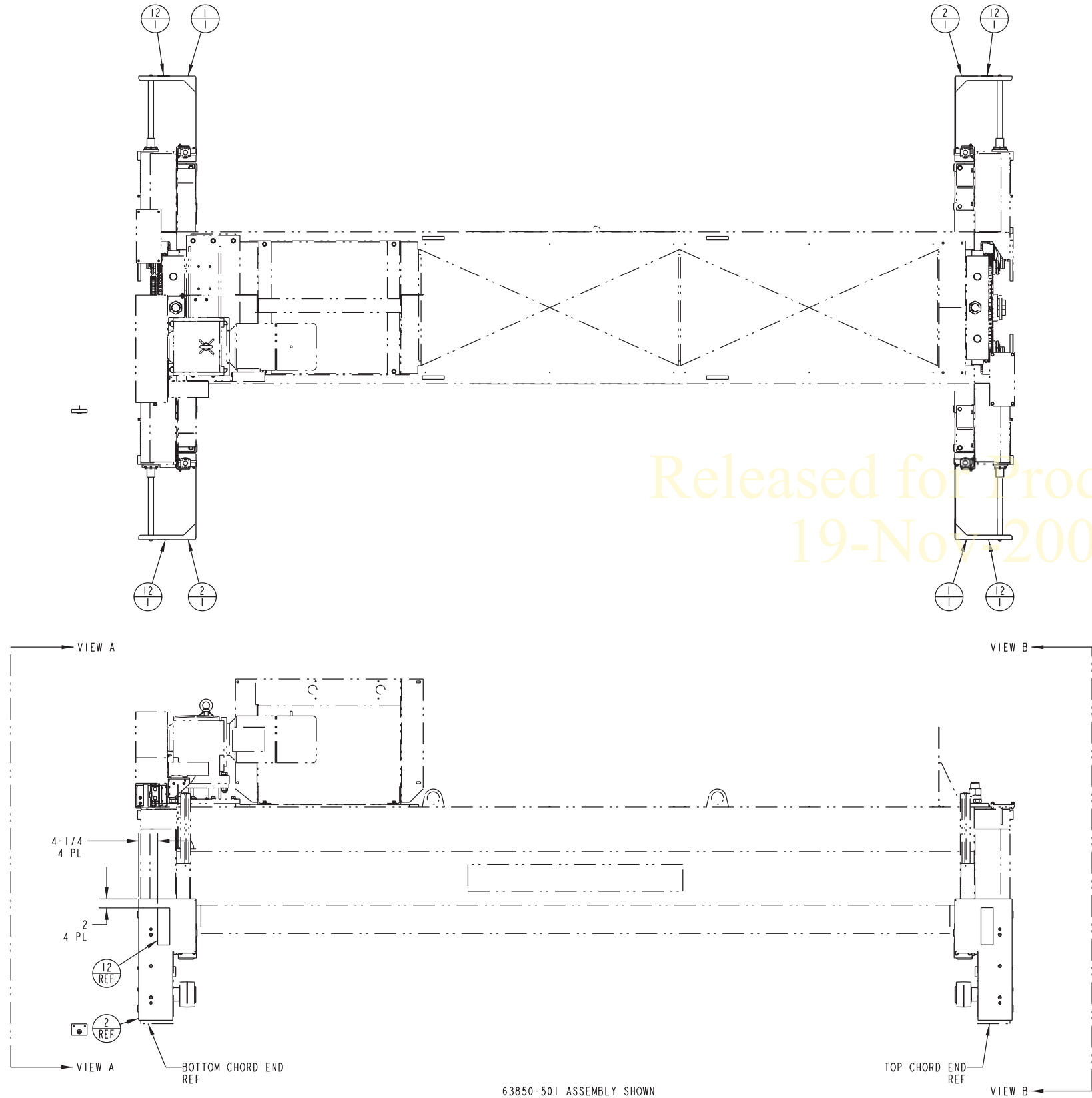
63850-501 ASSEMBLY SHOWN
