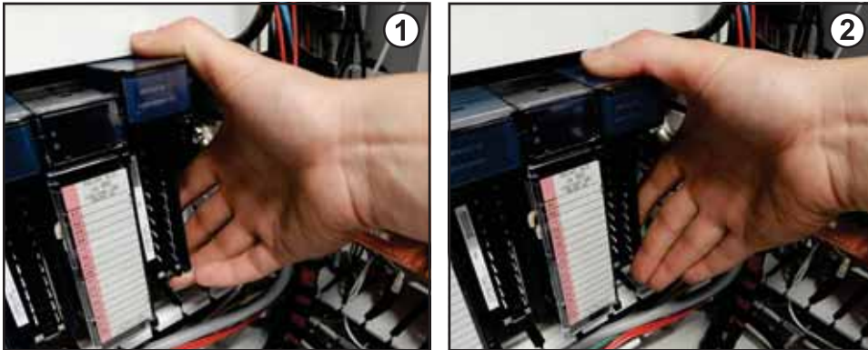
Figure 28: Placing the Module onto the Rack
