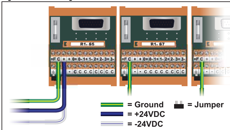
Figure 25: Connecting 24VDC
