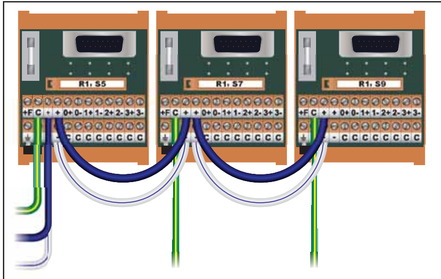
Figure 26: Jumping 24VDC from Module to Module
