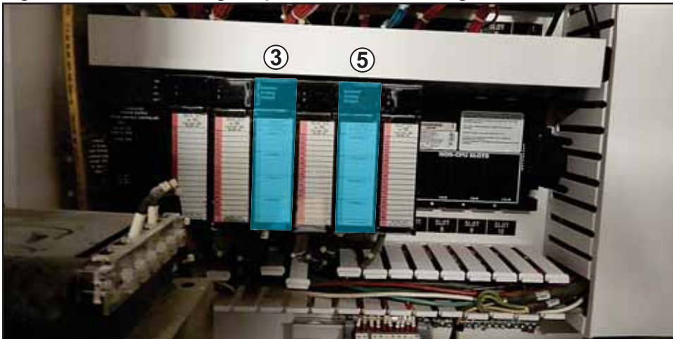
Figure 17: Horner Analog Output Modules in Carriage End
