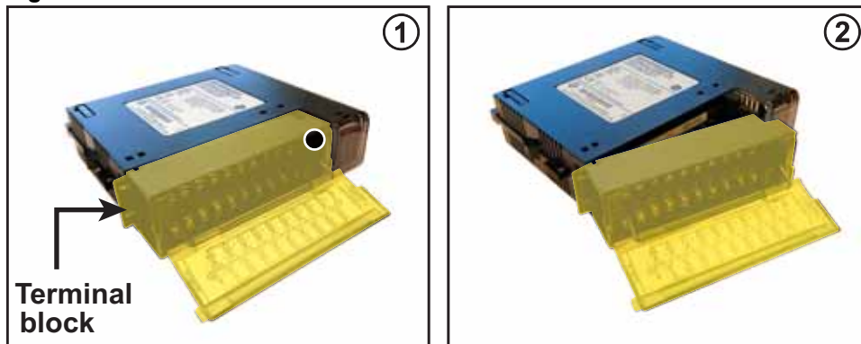
Figure 27: Terminal Block Removal
