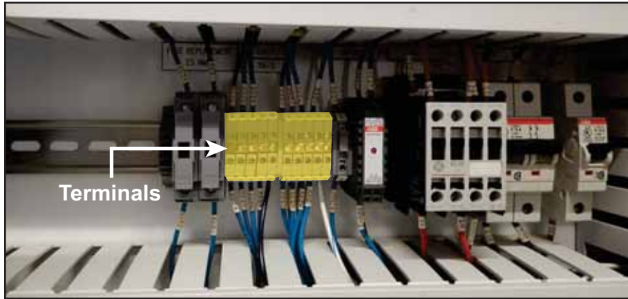
Figure 24: 24VDC Terminals
