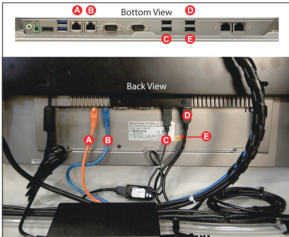
Figure 7: Connecting Cables to a BLADE Saw (computer models may vary)
