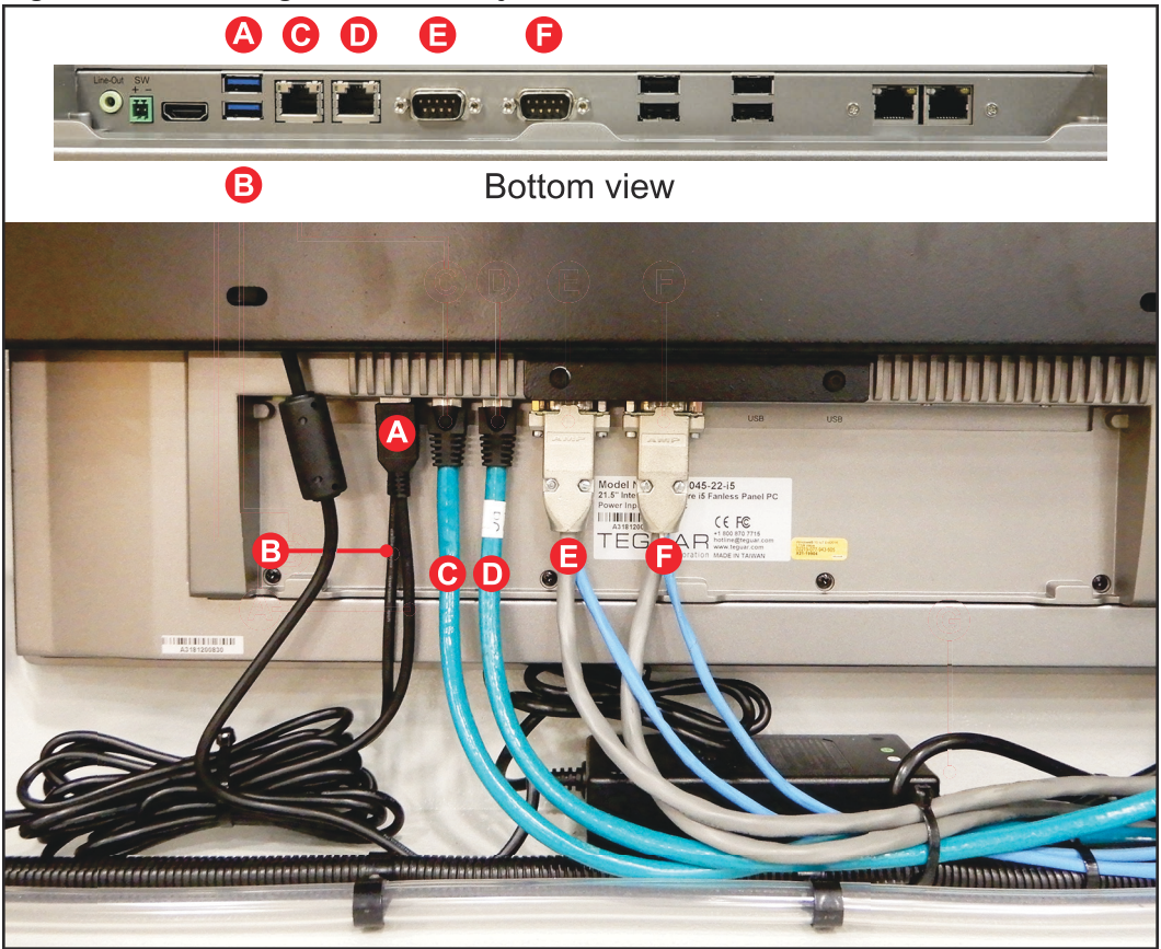
Figure 6: Connecting Cables for a Cyber A/T Saw
