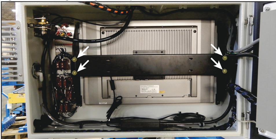
Figure 5: Installing the Teguvar Computer
