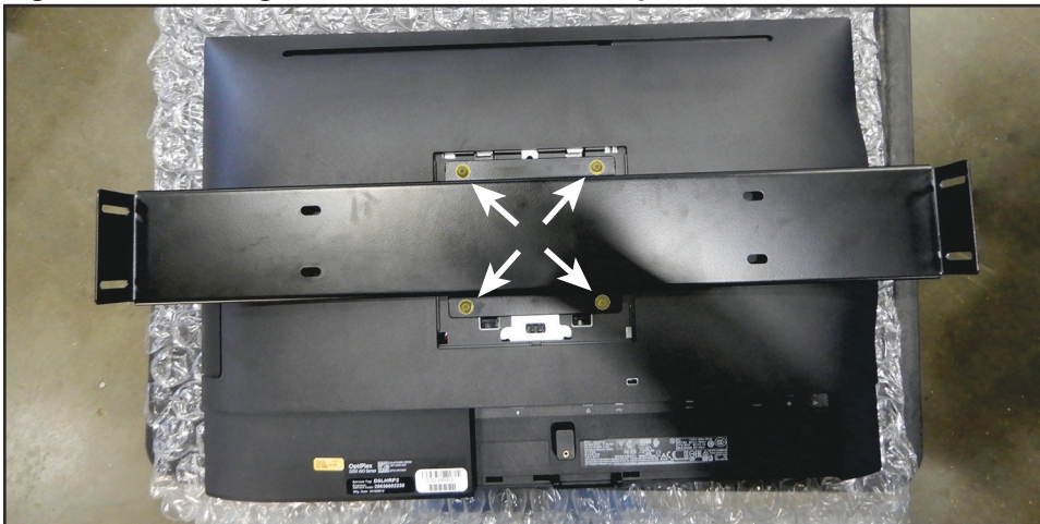
Figure 3: Removing the Bracket from the Computer
